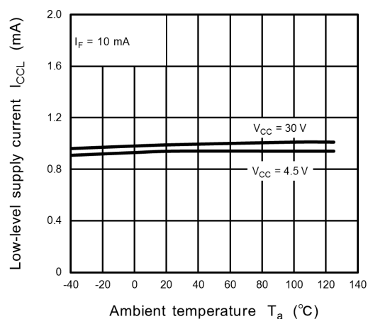
Fig. 13.2.5 I_{CCL} - T_a
