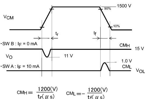
Fig. 13.1.7 Common-Mode Transient Immunity Test Circuit and Waveform
