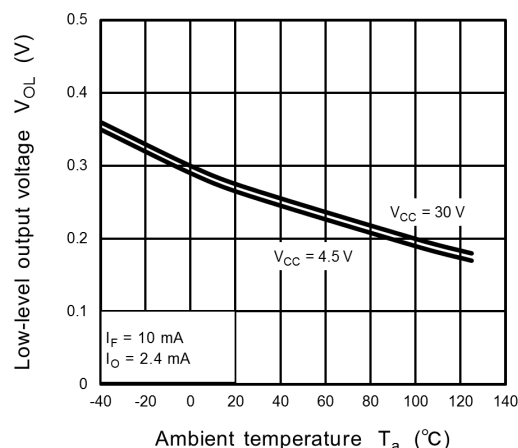
Fig. 13.2.8 V_{OL} - T_a
