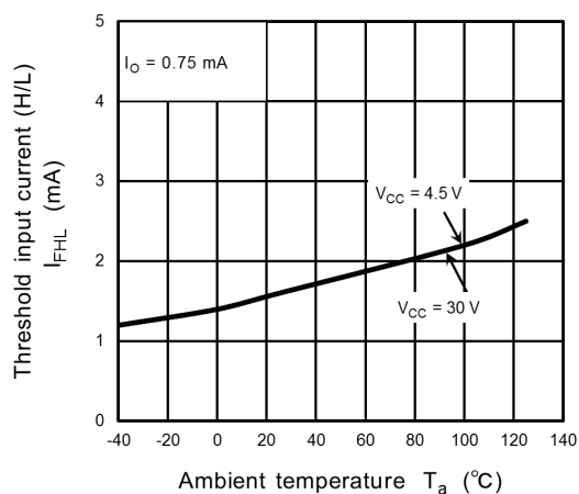
Fig. 13.2.3 I_{FHL} - T_a
