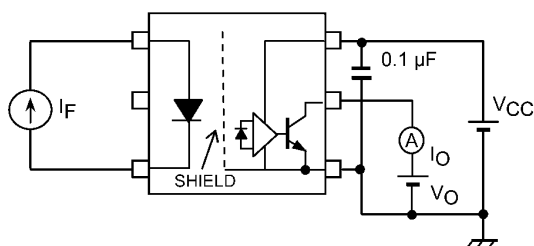
Fig. 13.1.5 I_O Test Circuit
